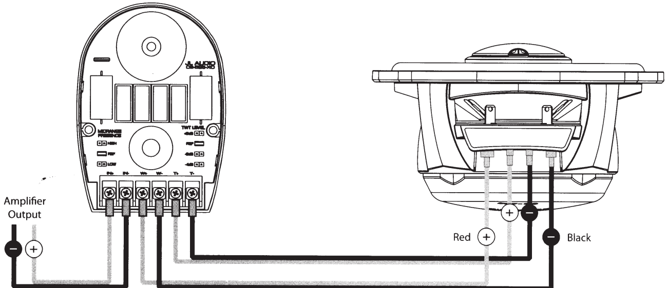
DIAGRAM B: Coaxial System Wiring
