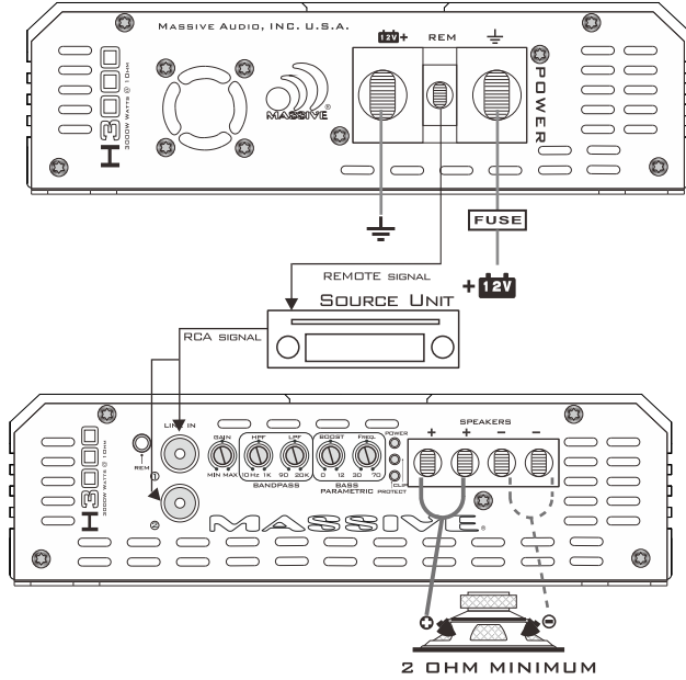
FIG 3. MONO AMPLIFIER WIRING H3000/H5000/H8000/12000
