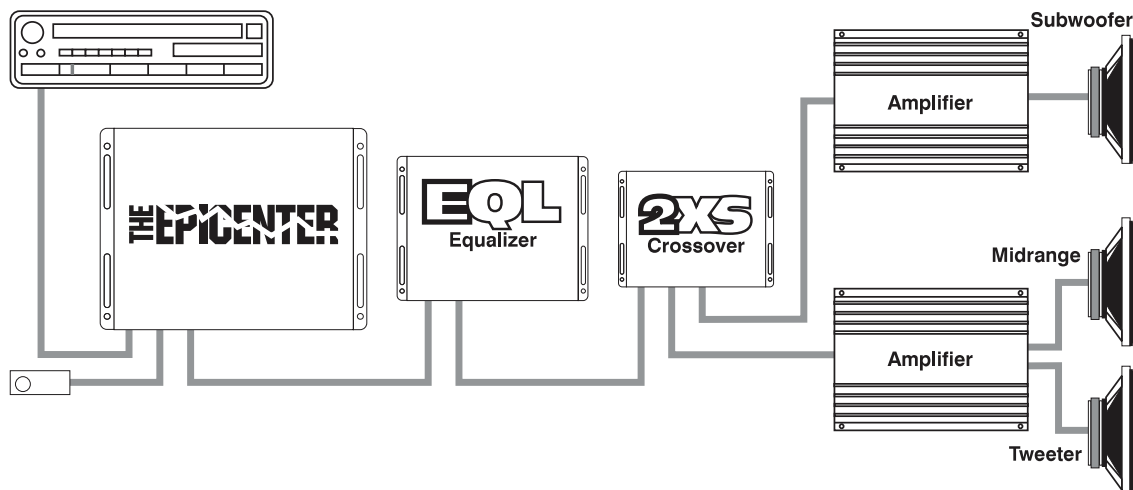
Figure 1: Quick Install
