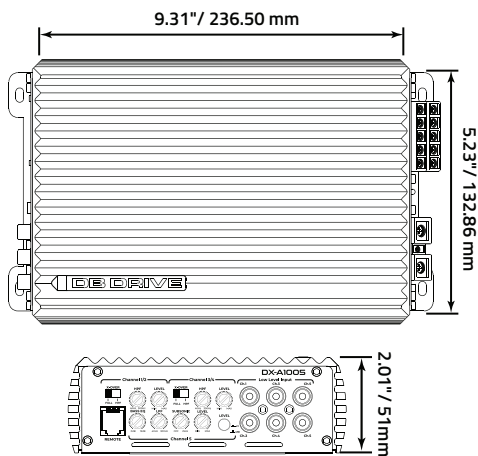
DX-A1005 Dimensions
