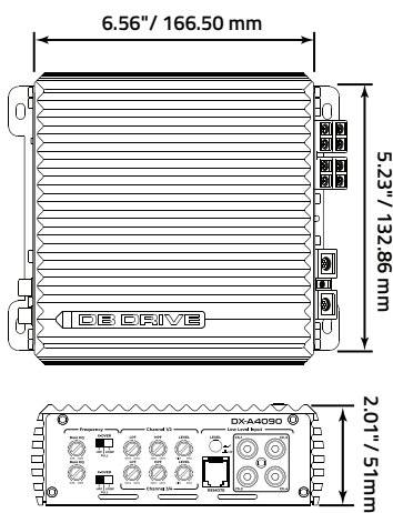
DX-A4090 Dimensions
