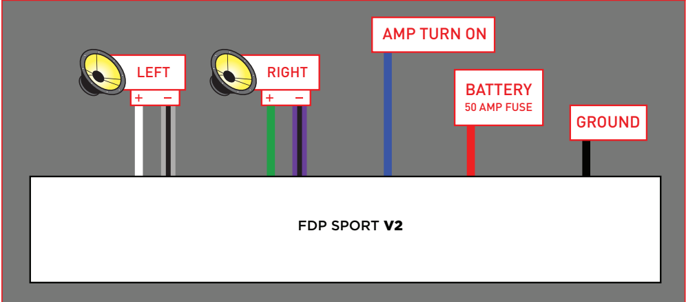
Figure 3B | 2 Channel Bridged Stereo Mode Wiring Diagram
