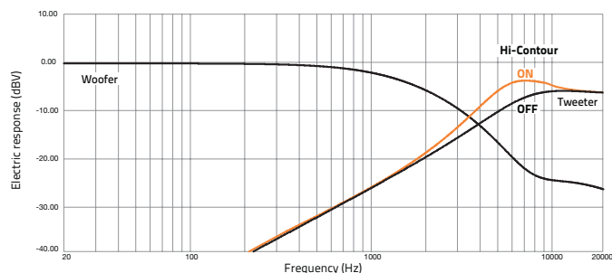
MLCX 165.3: Hi-Contour
