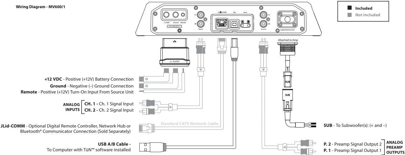
Wiring Diagram - MV600/1
