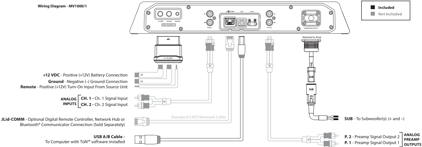
Wiring Diagram - MV1000/1
