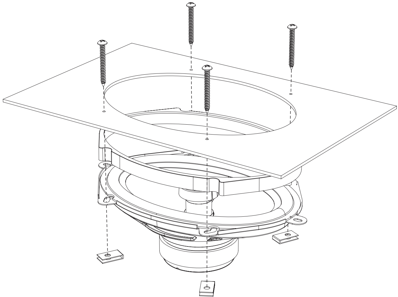
DIAGRAM A: Speaker Installation with Spacer Ring
