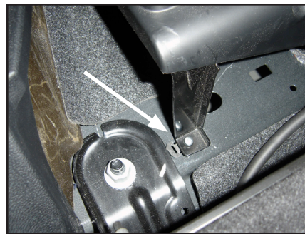
STEP 8 From behind the back seat, remove the two Phillips head screws that hold the front of the plastic tub in place, then remove the tub.
