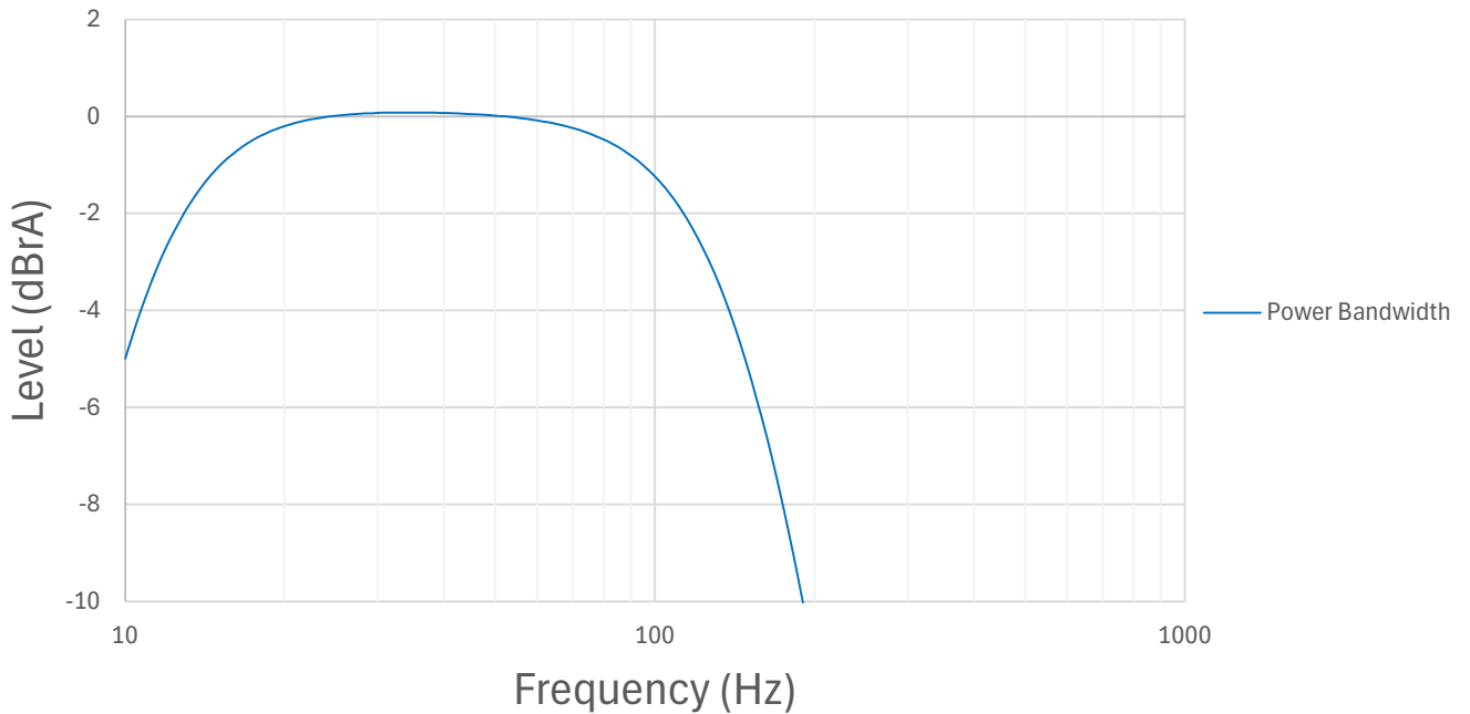
Power Bandwidth, re: Rated Power (400W @ 4Ω)
