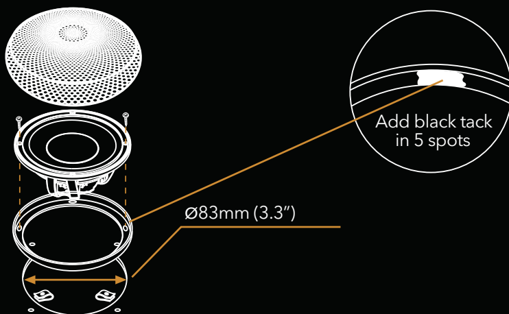
MS3 Midrange
