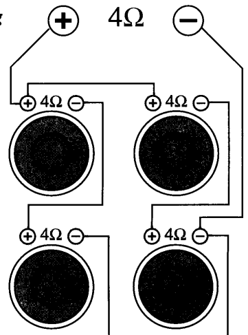
(4) 4 ohm SVC Speaker = 4 ohm Load
