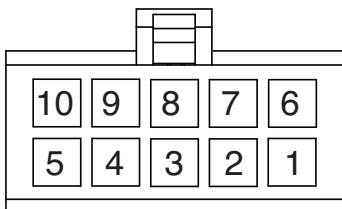
High-Level Input Harness (looking into the wire end)
