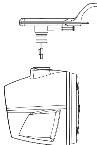
B - Connect wire to speaker
