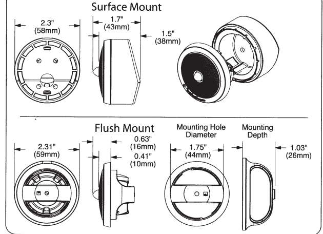
Mounting Options
