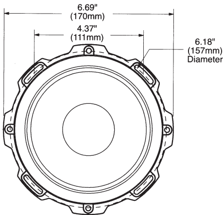
Woofer
