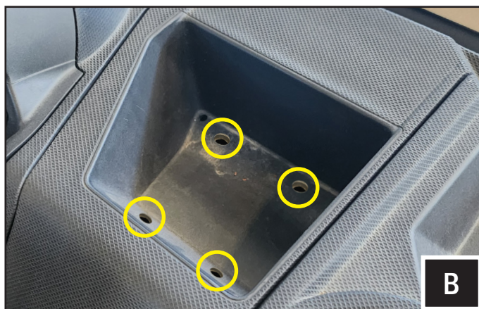
B. Drill (4) holes for the push rivets using a 5/16"holes drill bit.
