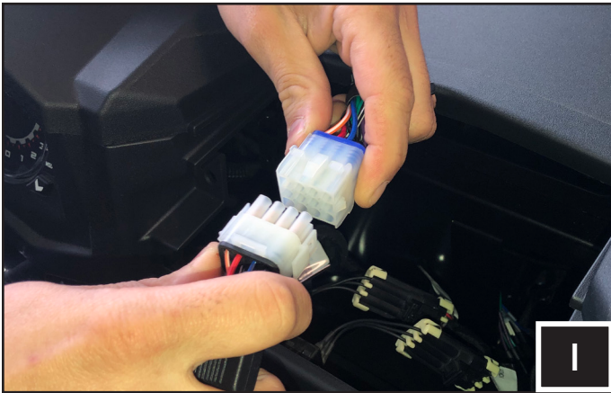
I. Connect the MR1 power harness to the radio harness. Plug in the provided universal antenna (B-H1249) if the vehicle does not have an antenna.
