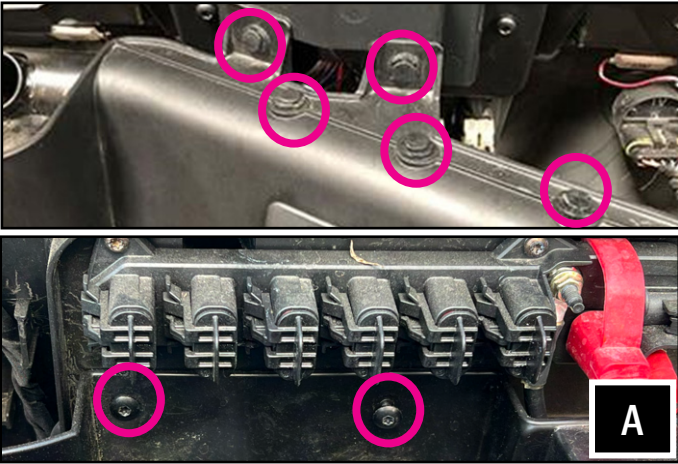
A. Remove the (5) push pins located on the plastic tray behind the radio. Extract (2) T25 screws located at the back of the plastic tray and below the bus bar, once extracted remove the plastic tray. Set aside the screws. The plastic tray will not be used in this installation.
