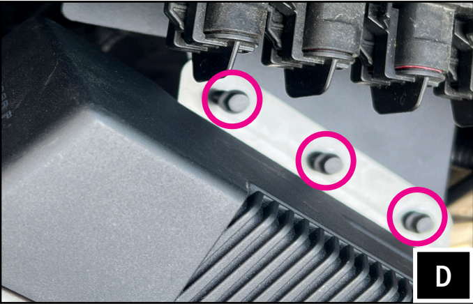
D. Secure the amp tray to the body bracket using the provided M6x12mm screws.
