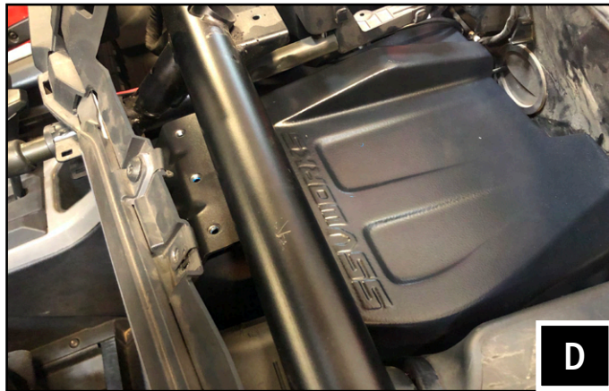
D. The top of the enclosure will tuck under the chassis cross bar. The bottom of the enclosure will rest above this edge of the firewall.
