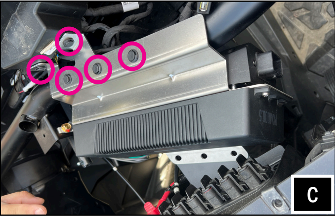
C. Line up the amp tray with the push pin holes and resuse the factory push pins to secure the amp tray.
