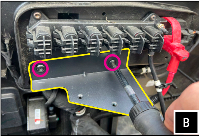
B. Attach the body bracket (B-A3451) under the bus bar using the factory screw bosses and T25 screws.
