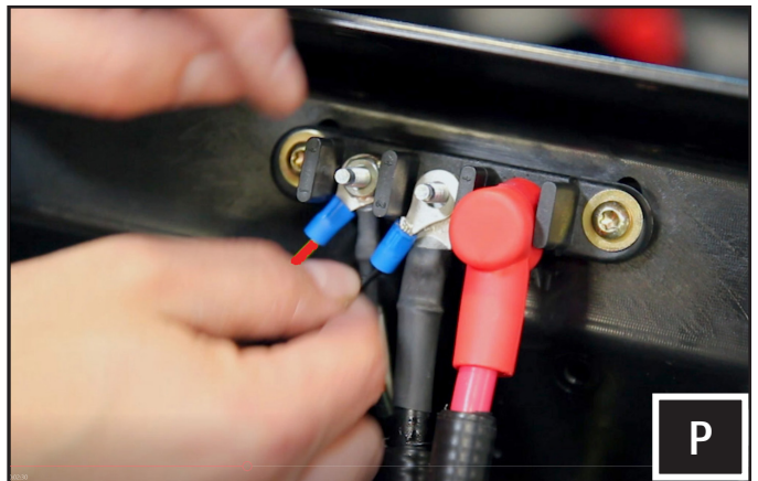
P. For vehicles with the terminal post style busbar, connect the ring terminals crimped on step I to the busbar.
