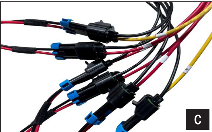
C. Route the pigtails connected to the devices power and ground wires to the RS6 switcher module location. Yellow wires are rated at 30A each and Red wires are rated at 25A each.
