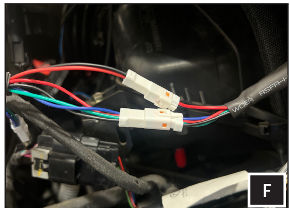
F. Make the audio and RGB connections to the tweeters and front speakers using the "Y" harness included in the kit.
