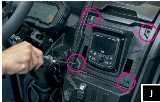
J. Secure the B-D2449 dash kit to the dash panel using 4 philips screws
