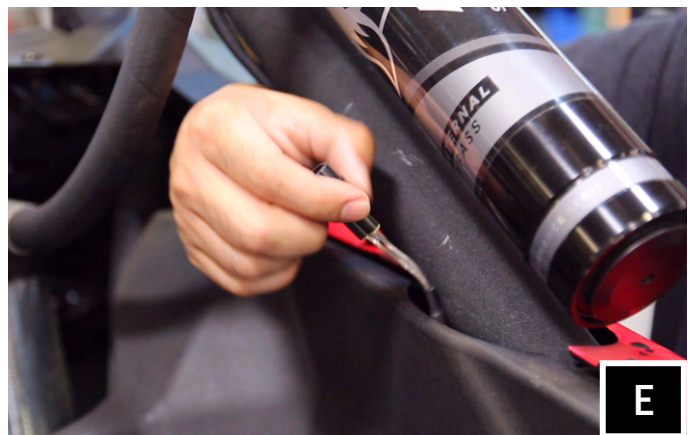
E. Route the Audio (B-1913 & B-H1912) and RGB extension harnesses (B-H2933 & B-H2934) along the factory wires in the engine compartment and pull up through the small space between the bed panel and cage tubing on both passenger and driver sides.
