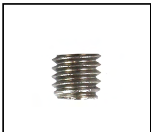
6. M6x1.0x6mm (3mm Allen Head) Screws x4
