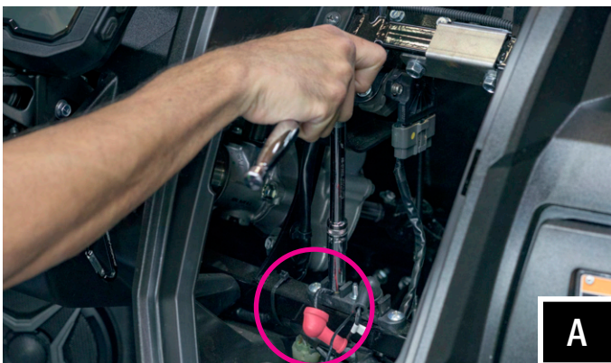
A. Attach the positive and negative ring terminals from B-H2367 harness to the accessory and ground posts mounted on the cross bar behind the dash
