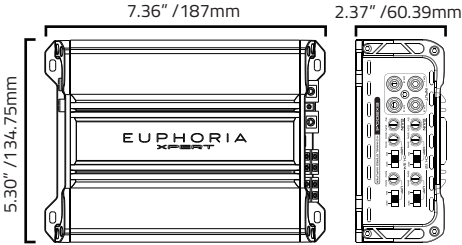
EX200.4 Dimensions
