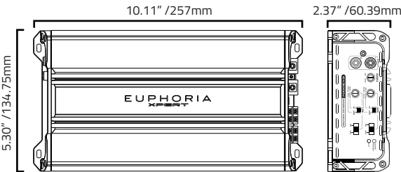
EX3000.1 Dimensions
