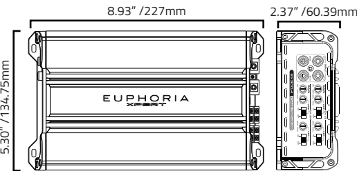
EX300.4 Dimensions
