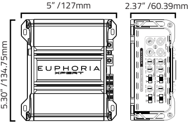
EX100.4 Dimensions
