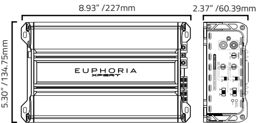
EX1500.1 Dimensions
